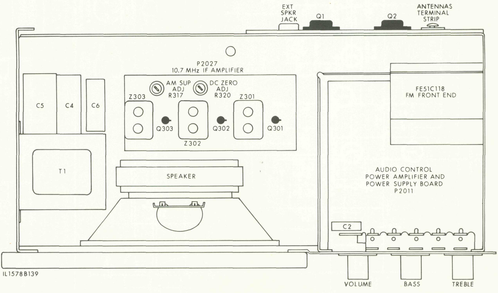
CHASSIS LAYOUT
